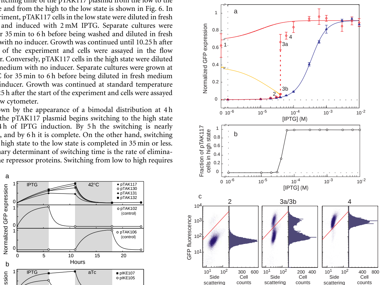
Figure 5 Toggle switch induction threshold. a , Steady-state gene expression after 17-h induction. The pTAK117 toggle plasmid (red circles) exhibits a quasi-discontinuous jump to the high state whereas the pTAK102 control plasmid (blue triangles) exhibits a sigmoidal induction curve. Point 1 is taken from separate experiments measuring the high state of pTAK117 with no inducer. Points 3a and 3b are the high and low modes of a bimodally distributed cell population. The bimodality occurs due to natural fluctuations in gene expression and the close proximity of the toggle switch to its bifurcation point. Theoretical curves are calculated from equation (1) with the term u/(1 + [\text{IPTG}]/K)^\eta , where K is the dissociation constant of IPTG from LacR and \eta is the cooperativity of IPTG binding, replacing u in the denominator of equation (1b). The red curves show the stable steady states and the orange curve shows the unstable steady state of the toggle. The blue curve shows the steady state of the IPTG-inducible control plasmid. Model parameters for the theoretical curves are \alpha_1 = 156.25 , \alpha_2 = 15.6 , \beta = 2.5 , \gamma = 1 , \eta = 2.0015 , K = 2.9618 \times 10^{-5} . b , Fraction of toggle cells in the high state at various concentrations of IPTG. The sudden switching to the high state is more clearly visible. High and low cell populations were divided as described for c below. c , Scatter plots (left plots) and histograms (right plots) illustrating the condition of the toggle cells at points 2, 3 and 4 (of a ) near the bifurcation point. High-state and low-state cell populations are divided by the red line in the scatter plots. The two states of the toggle are clearly evident in the bimodally distributed cells (point 3).
